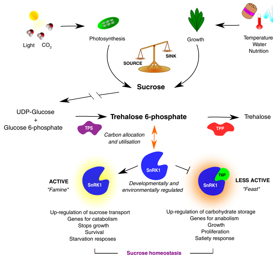
Fig. 3. Sugar signalling via trehalose 6-phosphate (T6P)/SnRK1 interactions. The sucrose status of plant tissue is relayed through T6P to SnRK1. The activity of SnRK1 which is inhibited by T6P determines gene expression for starvation or satiety responses and maintains sucrose homeostasis. There is strong cell and developmental specificity of expression of genes regulating T6P content. Cell specific changes in T6P may enable modification of plant process and particularly productivity and resilience of crops.
